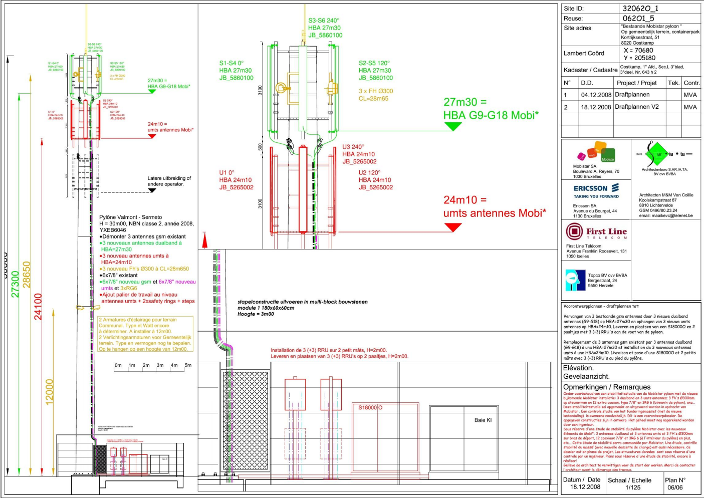
H0800 Front View, v2
